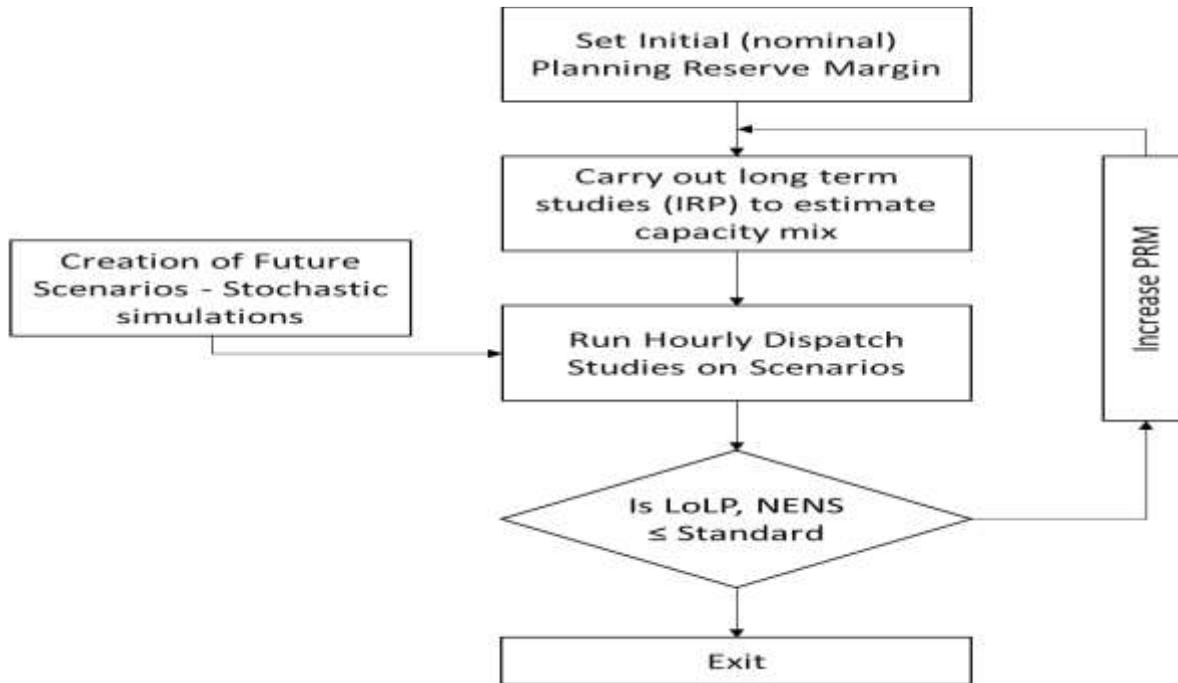
Flow Chart of Optimal Reserve Margin Study
